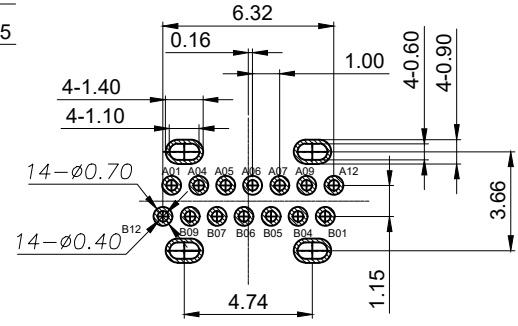
RECOMMENDED P.C.B. LAYOUT (俯视图) TOLERANCE UNSPECIFIED ±0.05mm
